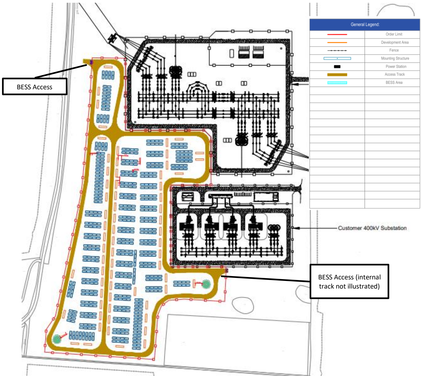
Figure 2.1 Illustrative Scheme Layout
